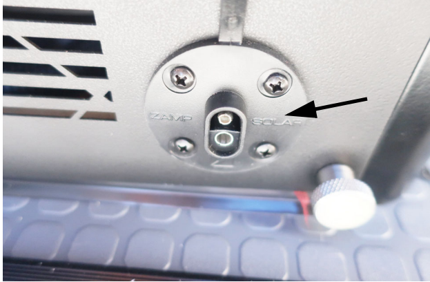
Single Solar Port (Located behind driver’s side rear door.) -Typical View
