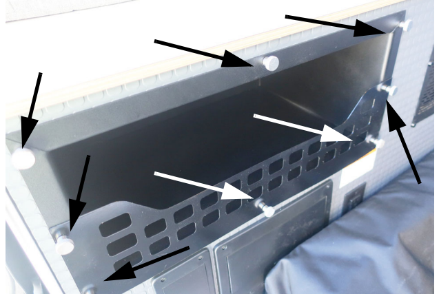
Remove 8 twist screws to access inside panel to reveal slot to add additional batteries. -Typical View
