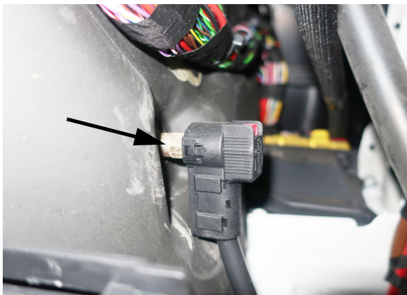
Chassis Battery Connector (Located to the right of the accelerator pedal behind access panel)
