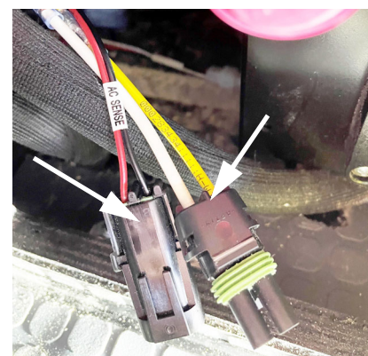
Red/Black wires labeled AC Sense. Yellow wire labeled WJ, White wire labeled JX. -Typical View
